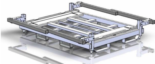
FOLD OUT ALONG DECK FOR LOADING
