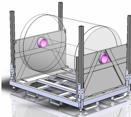
SUSPENDED ROLL W/ CORE PLUGS
